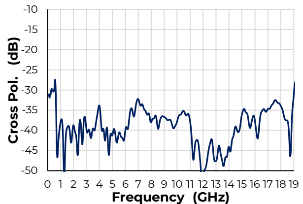
Cross Polarization
