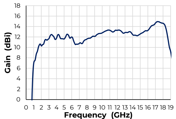
Gain
